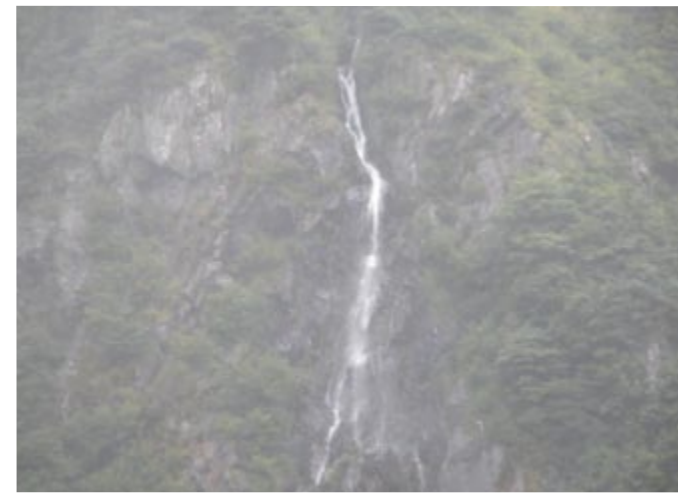
Waterfall blown upstream by wind gust
